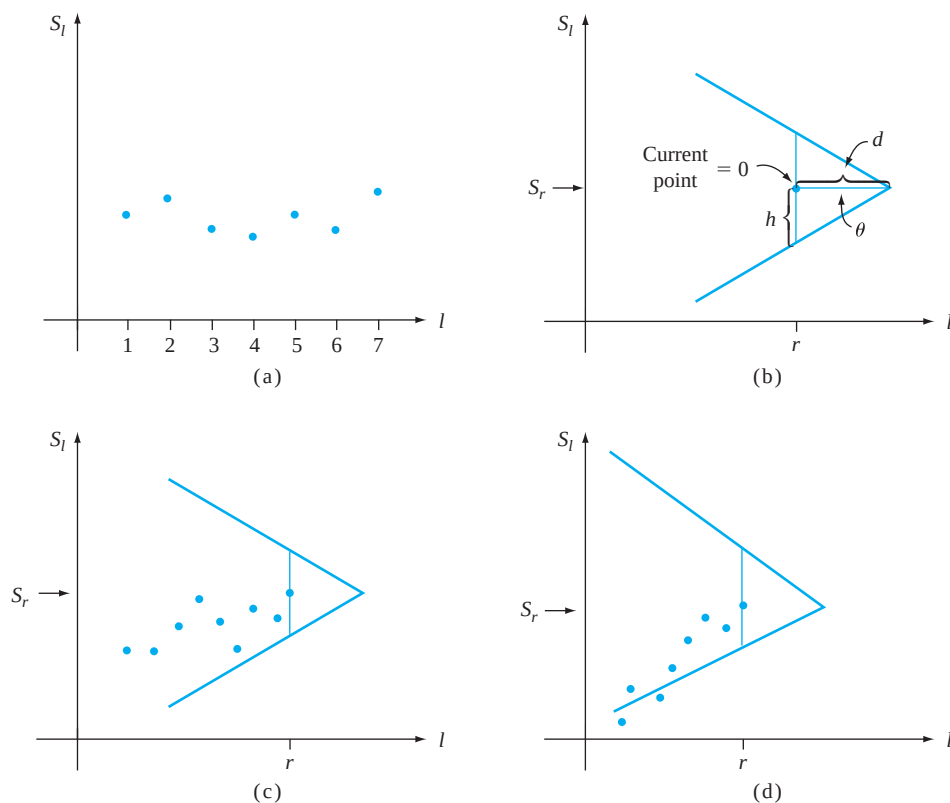
Figure 16.7 CUSUM plots: (a) successive points (l, S_l) in a CUSUM plot; (b) a V-mask with O = (r, S_r) ; (c) an in-control process; (d) an out-of-control process
