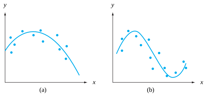
Figure 13.10 (a) Quadratic regression model; (b) cubic regression model
