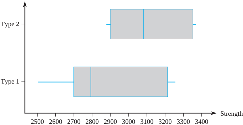
Figure 9.3 A comparative boxplot of the tensile-strength data
