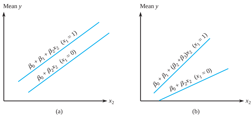
Figure 13.14 Regression functions for models with one dummy variable ( x_1 ) and one quantitative variable x_2 : (a) no interaction; (b) interaction
