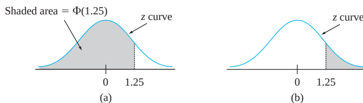
Figure 4.15 Normal curve areas (probabilities) for Example 4.13
